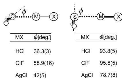
Figure 1. Angular geometries of several \text{H}_2\text{Y}-\text{M}-\text{X} compounds; \cdots indicates the local C_2 axis of the \text{H}_2\text{O} or \text{H}_2\text{S} subunit.
